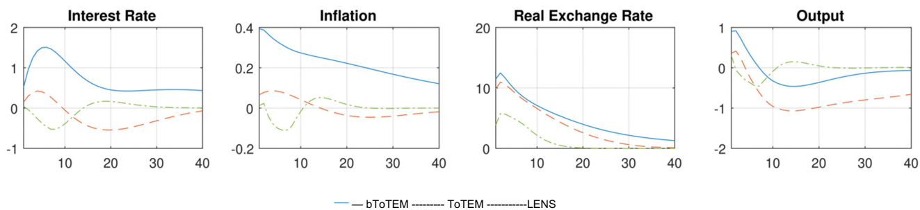
Figure E.3: Impulse response functions: ROW interest rate shock
