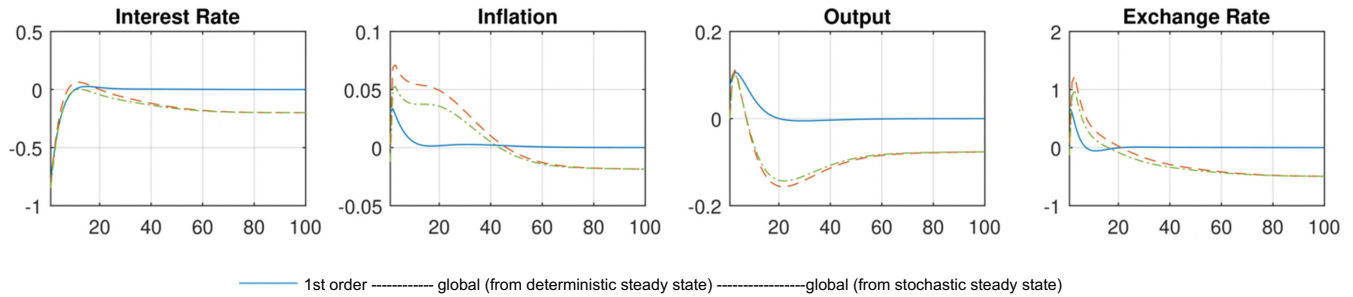
Figure 10: Modified experiment 2. Linear perturbation and two global solutions, one of which starts from the deterministic steady state and the other starts from the stochastic steady state (variables are shown in deviations from the 3% deterministic steady state)
