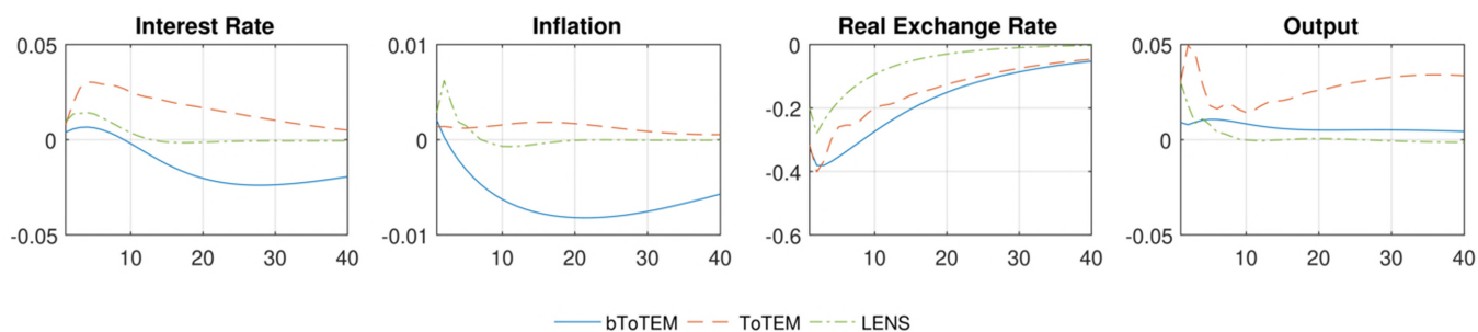
Figure E.1: Impulse response functions: ROW commodity price shock
