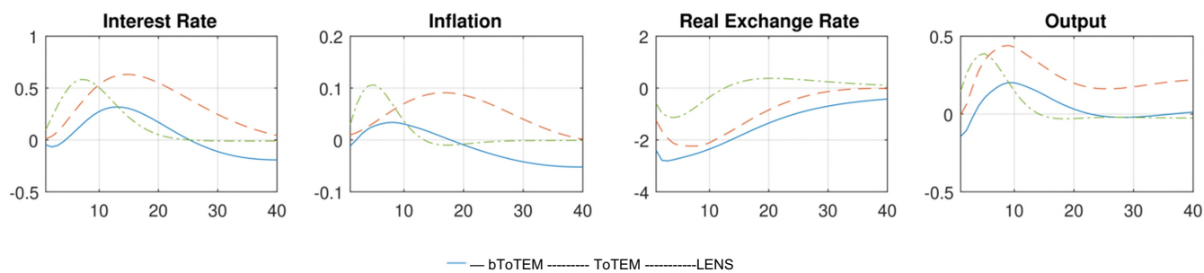
Figure E.2: Impulse response functions: ROW demand shock
